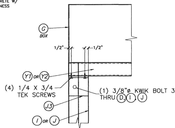
CASE II : ELEVATION X1
