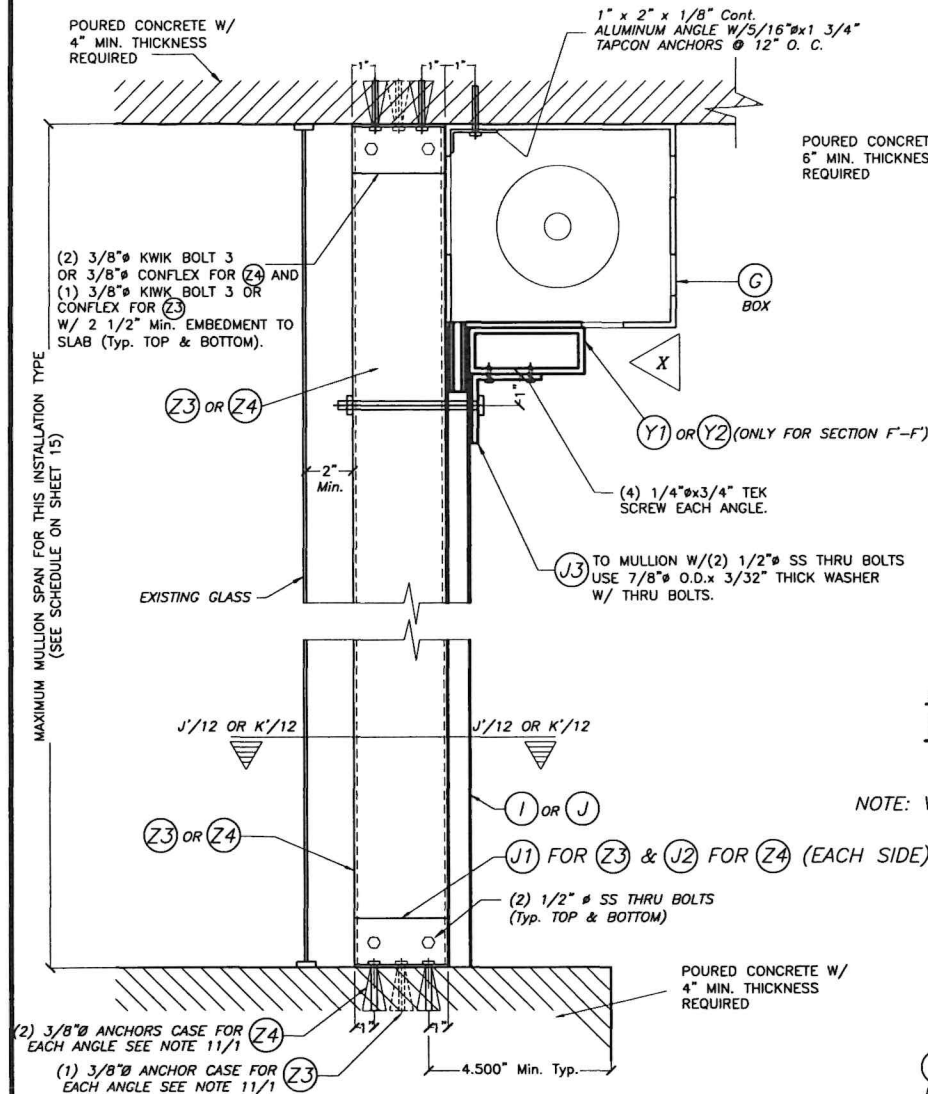
CASES III & IV : FLOOR/CEILING MOUNTING : SECTION F-F W/O HEADER & SECTION F'-F' W/HEADER
