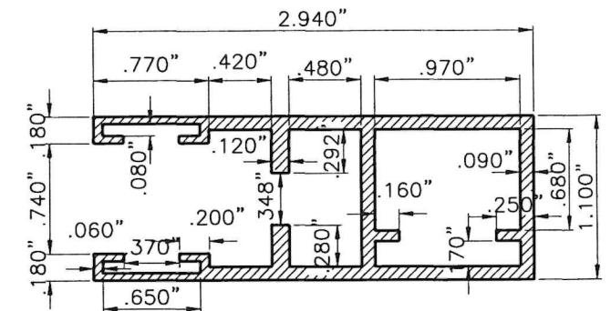
J SIDE RAIL TYPE 3
