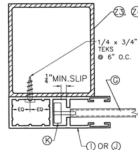
SECTION J''-J'': MULLION MOUNT (FACE MOUNT)
