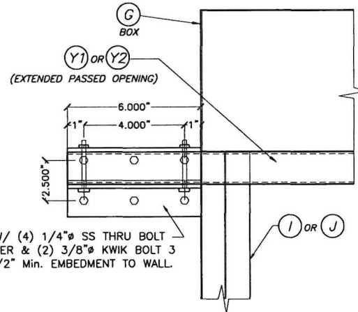
CASE II : ELEVATION X2
