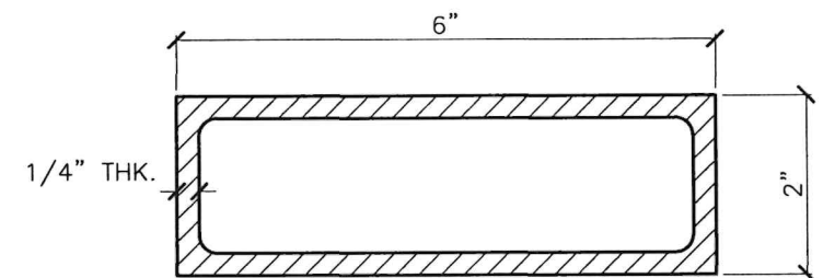
(Y2) 6"x2"x1/4" HEADER ALUMINUM 6061-T6 ALLOY & TEMPER
