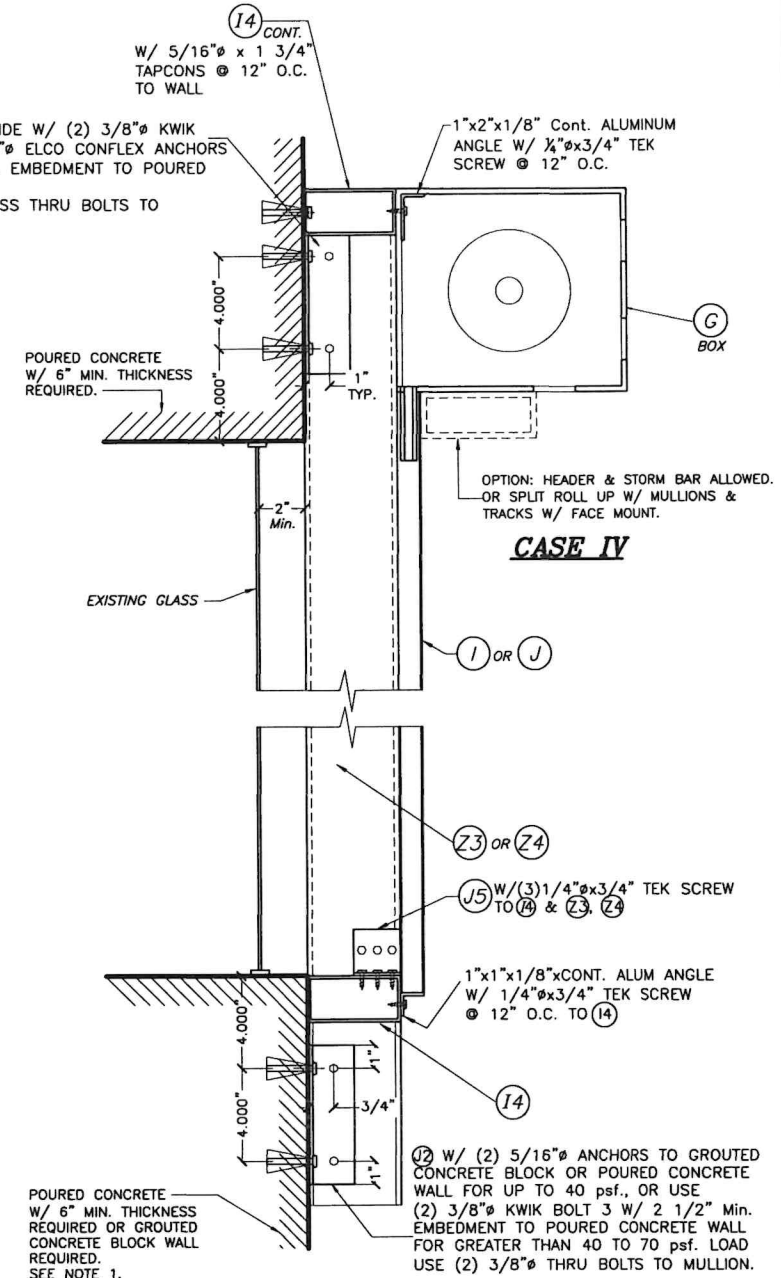
CASES III & IV : WALL MOUNTING: MULLION CONNECTION AT TOP & BOTTOM: SECTIONS I - I' (W/O HEADER) & I' - I' (W/HEADER)
