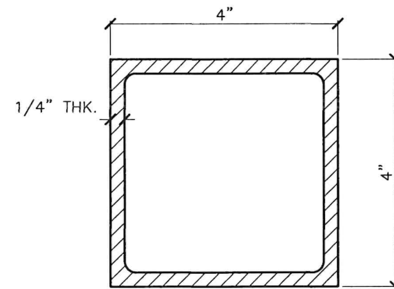
(Z3) 4"x4"x1/4" MULLION ALUMINUM 6061-T6 ALLOY & TEMPER
