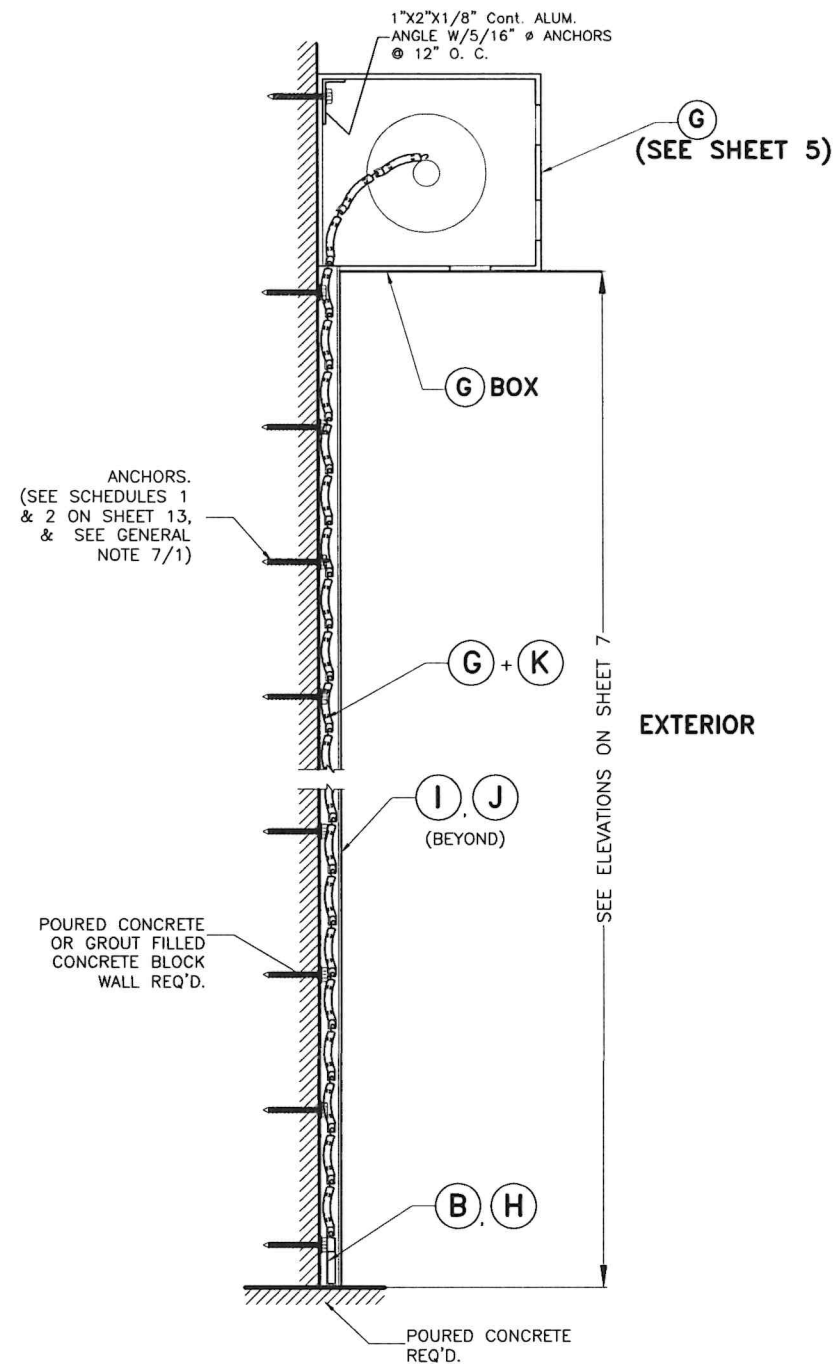
CASES I, II, III & IV SECTION A-A (WALL MOUNTED) SCALE 1-1/2"=1"
