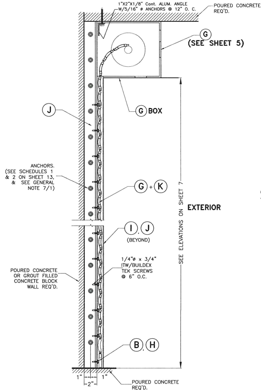
CASES I, II, III & IV SECTIONS B-B (TRAPPED MOUNTED) SCALE 1-1/2"=1"
