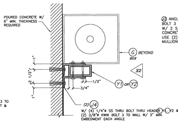
CASE II : HEADER ANCHORAGE METHOD 2 WALL MOUNTING : SECTION H - H
