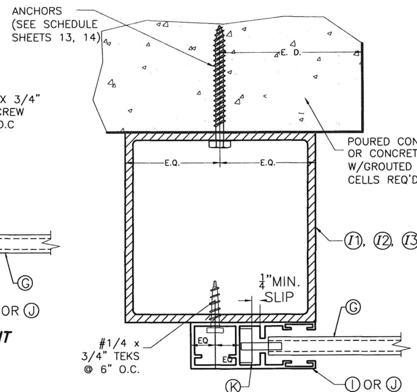
SECTION L-L: BUILD-OUT MOUNT
