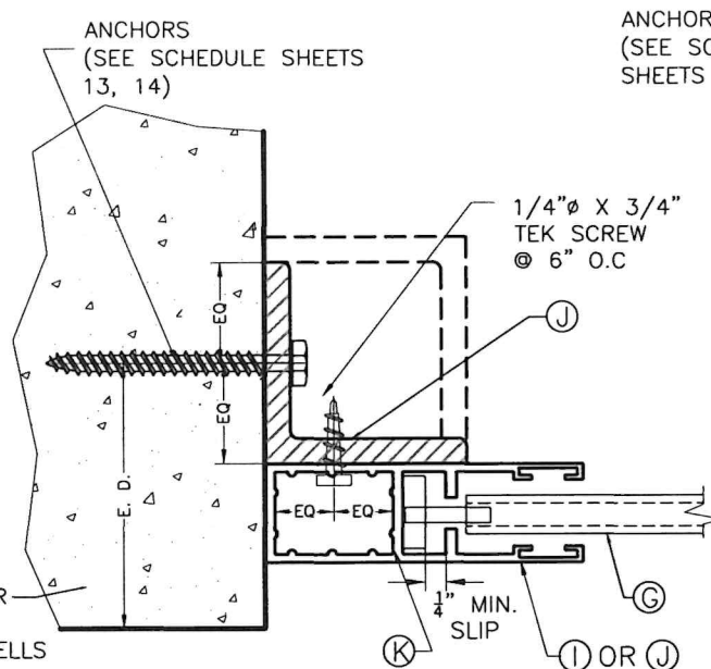
SECTION K-K: INSIDE MOUNT
