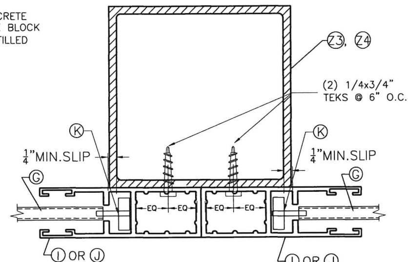
SECTION J'-J': MULLION MOUNT FACE MOUNT
